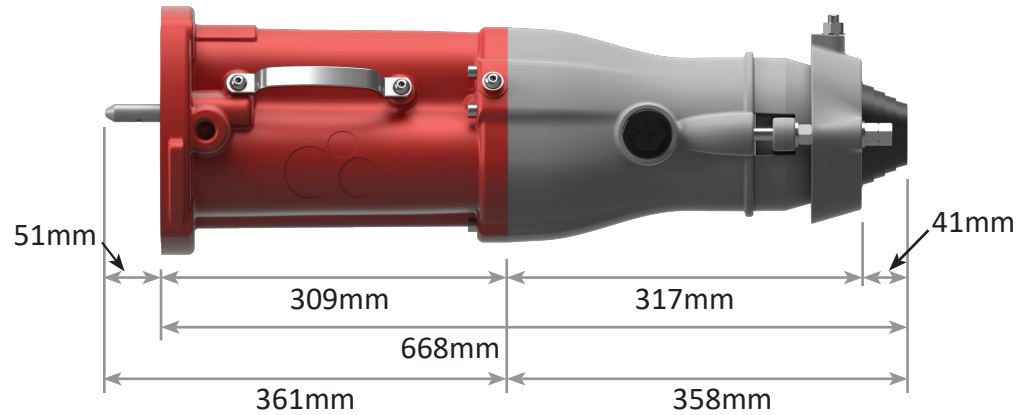
Side View (Armoured)
