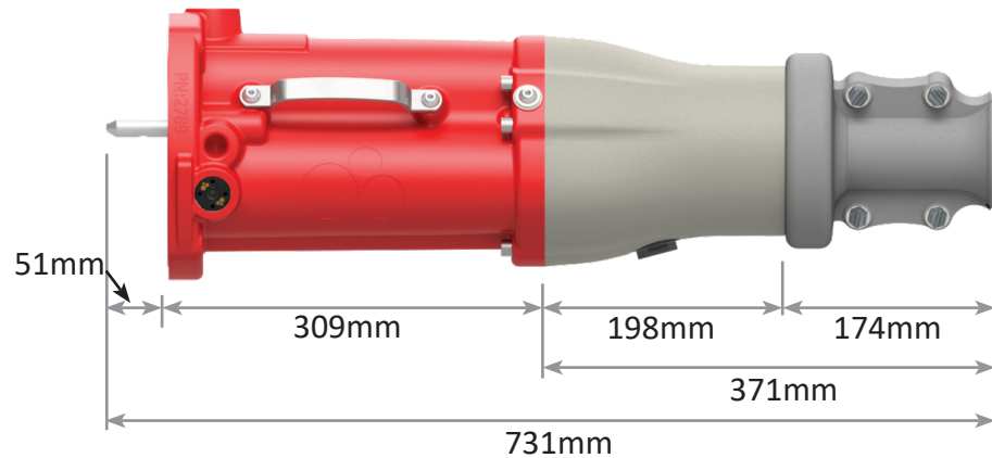
Side View (Unarmoured)
