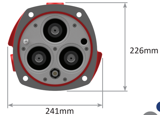
Front View with Live Line Indicators
